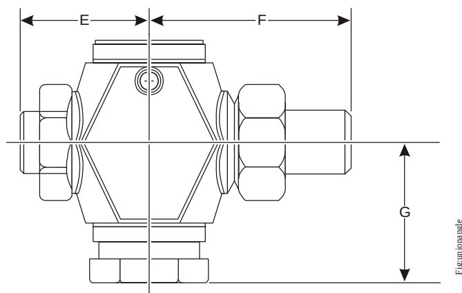
Figure 5: Two-Way Union Angle Valve Dimensions
